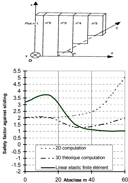
Fig 5.7: Safety factors against sliding. (from Ref. 5.7) Comparison among different 2D and 3D approaches
